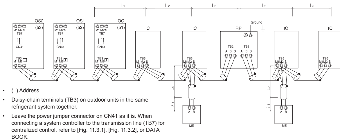
[Fig. 11.3.3] Combination of outdoor units and transmission booster unit
